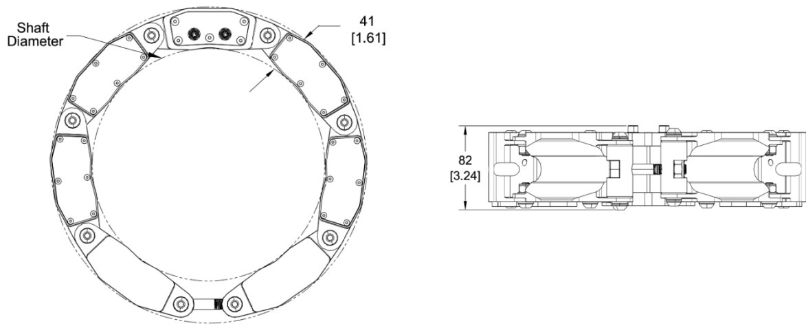
TX50 Collar Dimensions (mm [inch])
