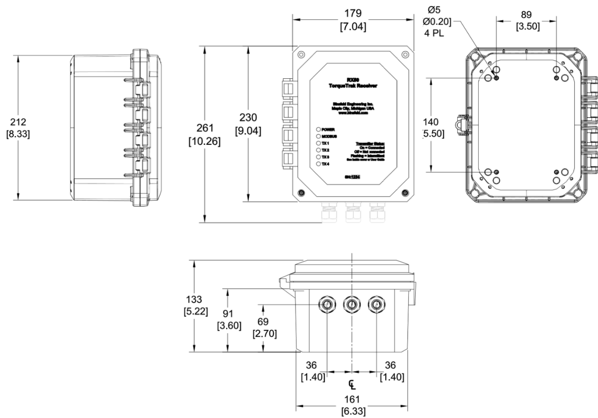
RX50 Receiver Dimensions (mm [inch])
